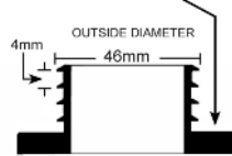
Thread Cutaway
