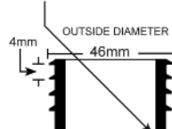
Thread Cutaway
