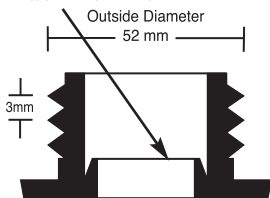
Thread Cutaway
