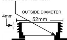
Thread Cutaway
